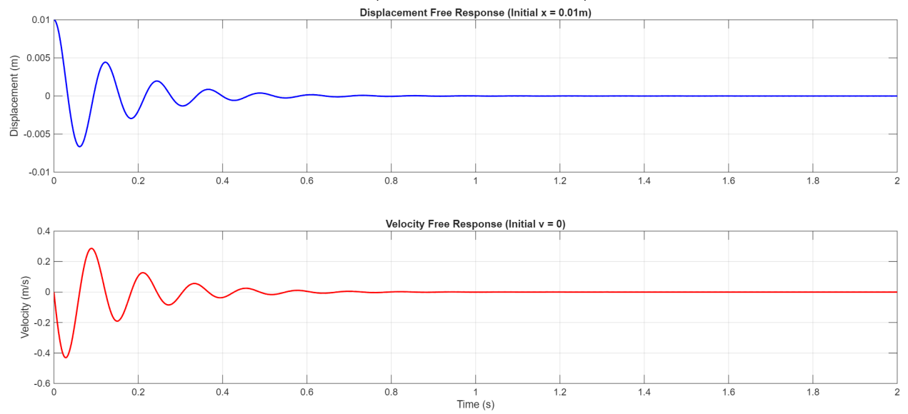
Part 2d: Free Response of the Truck with Initial Displacement
