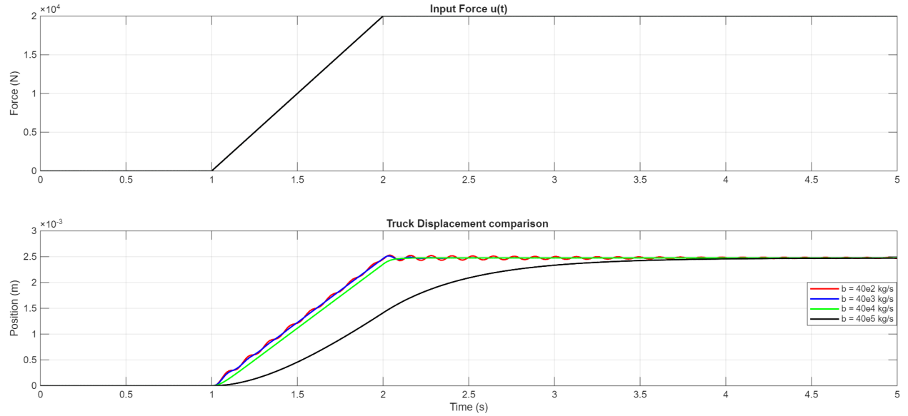
Part 2c: Comparison of Truck Displacement for Different Damping Coefficients
